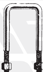
15 - 722011 \varnothing 14 \times 60 \times 130 16 - 722555 \varnothing 14 \times 60 \times 140 17 - 722556 \varnothing 14 \times 60 \times 150 18 - 722557 \varnothing 14 \times 60 \times 160
