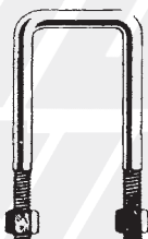
14 - 722512 \varnothing 14x70x150 15 - 722513 \varnothing 14x70x170 16 - 722514 \varnothing 14x70x190
